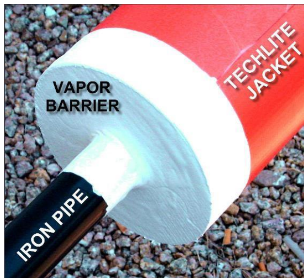
Photo 3: Special fittings
