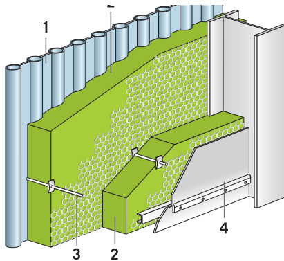
Diagram of a boiler insulation system with wired mats
