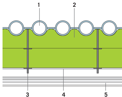
Diagram of a boiler insulation system with ProRox Wired Mats with a gap between the insulation and sheet cladding
