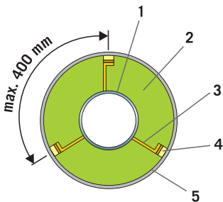
1. Pipe - 2. ProRox Insulation - 3. Spacer - 4. Thermal dividing layer - 5. Support ring - 6. Cladding
