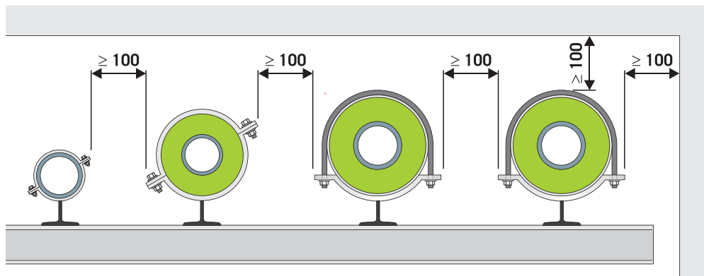
Minimum distances between insulated pipes (dimensions in mm)
