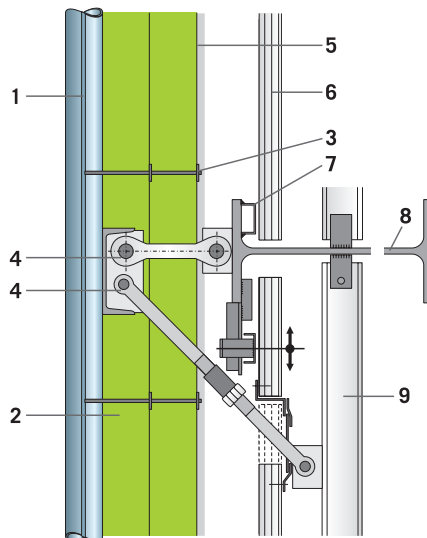
Buckstays exposed to cold on a boiler wall
