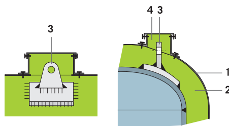
Insulation of a crane hook
