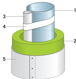
1. Pipe - 2. Insulation: ProRox Pipe Sections - 3. Tracing - 4. Binding tape - 5. Cladding
