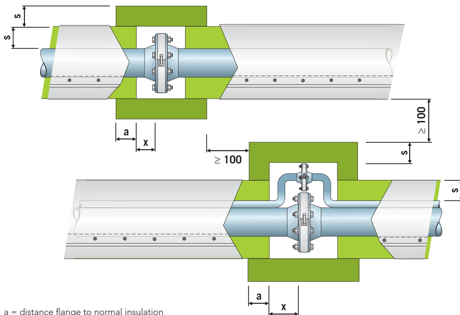
Minimum distances within range of pipe flanges (dimensions in mm)
