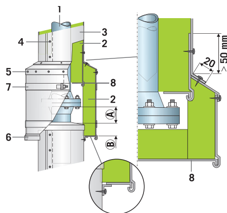
1. Pipe - 2. Insulation: ProRox Wired Mats - 3. Sheet - 4. Sheet-metal screw or rivet - 5. Rain deflector - 6. Lock washer - 7. Straps - 8. Lock washer - B \geq 50 \text{ mm} - A = \text{Screw length} + 30 \text{ mm}
